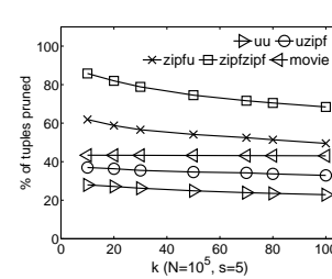
Fig. 13. Attribute-level: Pruning of A-ERank-Prune.
