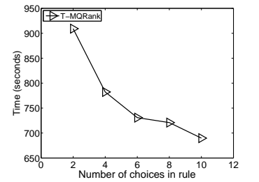
Fig. 14. Tuple-level: Effect of \psi for median and quantile ranks.
