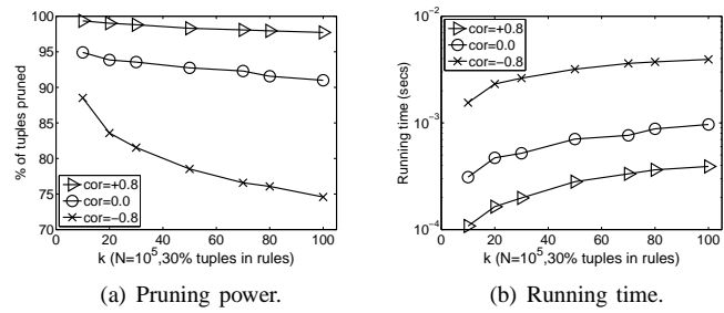
Fig. 8. Impact of different correlations on T-ERank-Prune.
